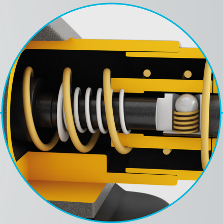
PRECISE FOAM ADJUSTOR Saves foam
